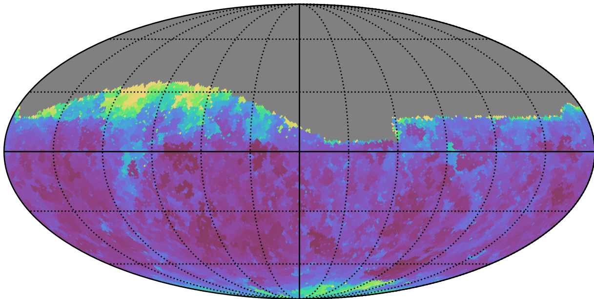
noroll_mjdp180_v3.4_10yrs Yr 1 i band: Min seeingEff
