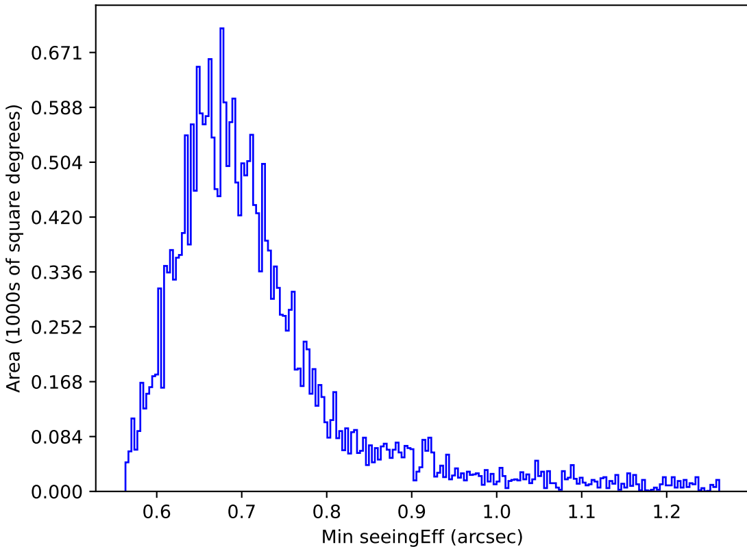
noroll_mjdp180_v3.4_10yrs Yr 1 i band: Min seeingEff
