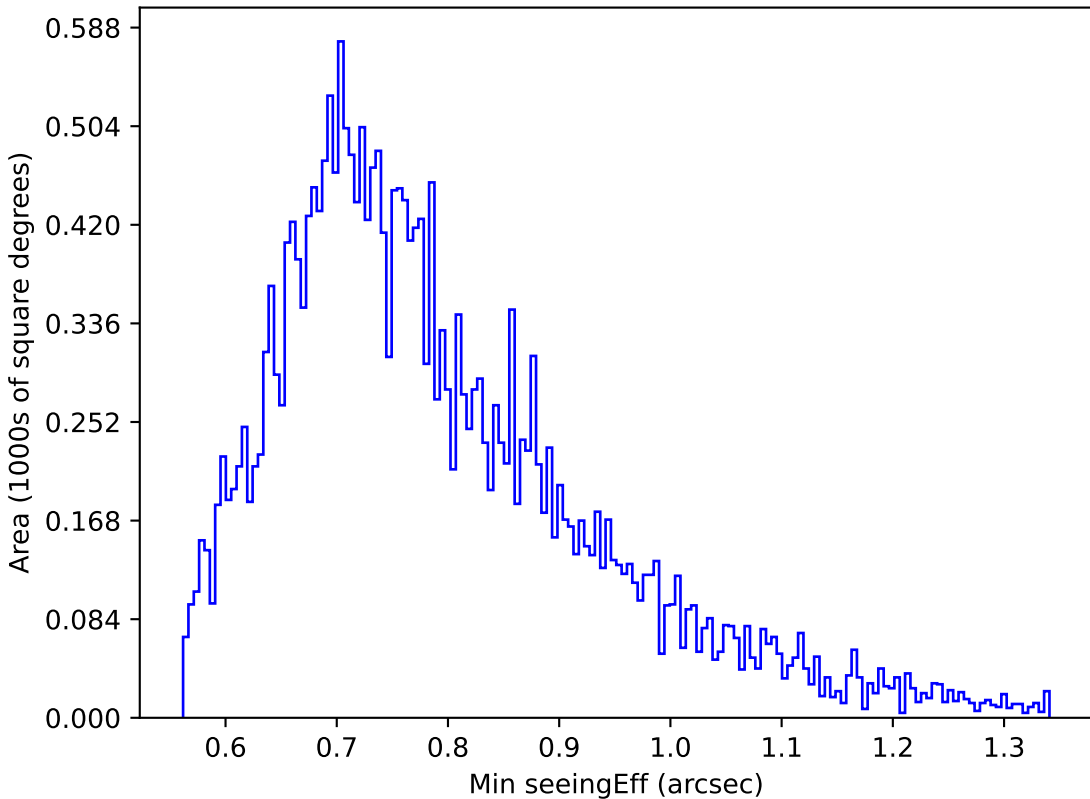
noroll_mjdp180_v3.4_10yrs Yr 1 g band: Min seeingEff
