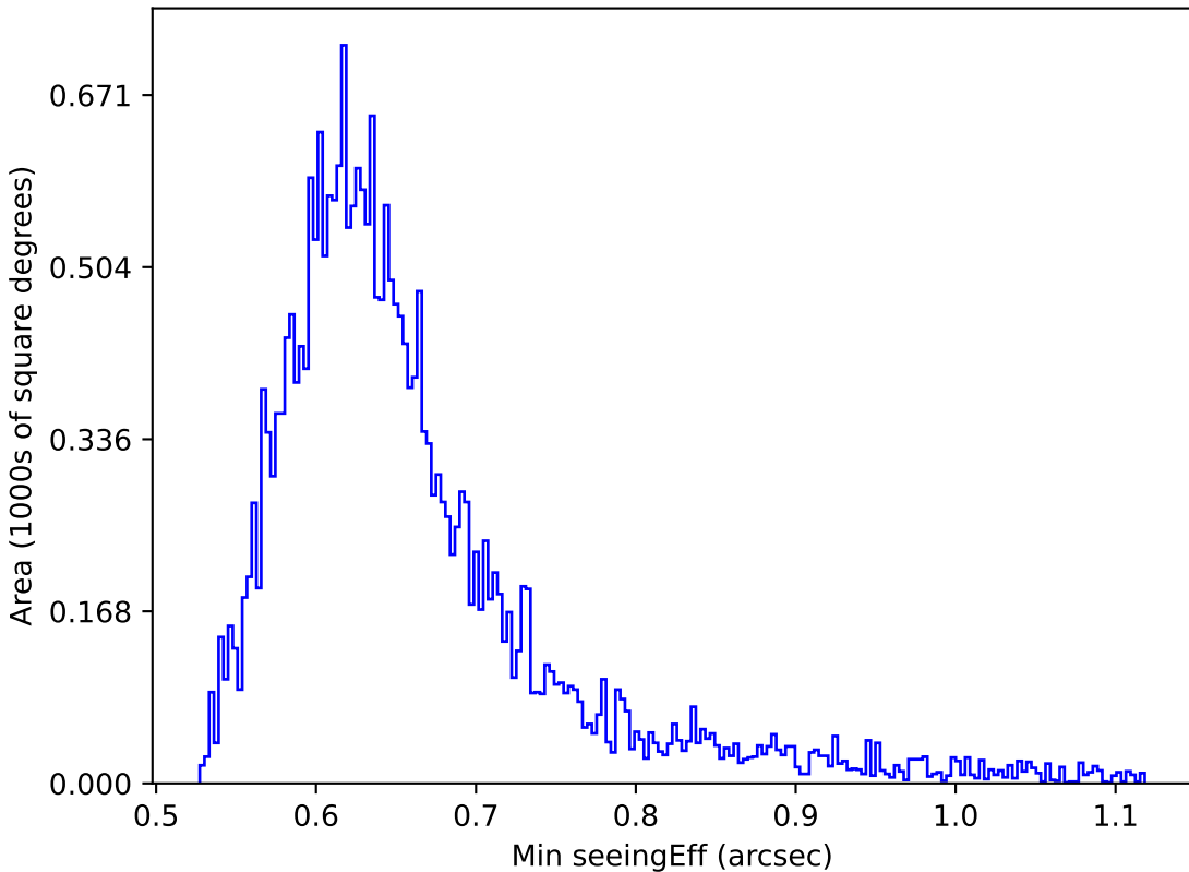
noroll_mjdp180_v3.4_10yrs Yr 1 all bands: Min seeingEff
