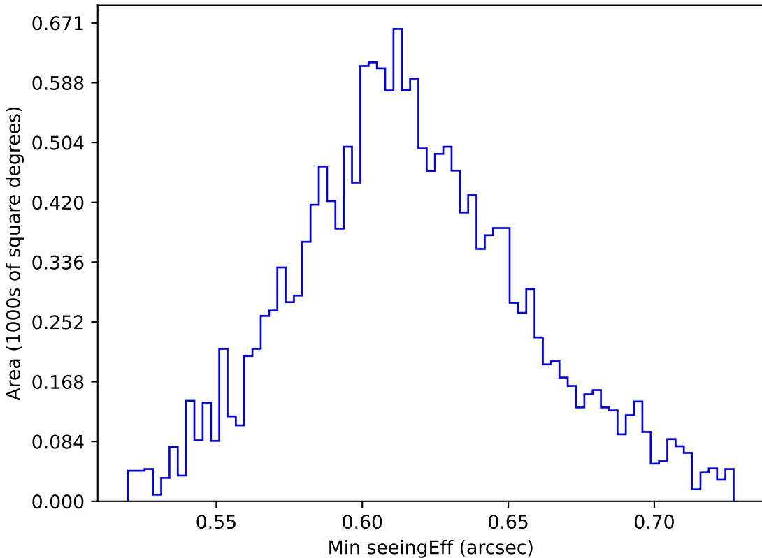
noroll_mjdp180_v3.4_10yrs WFD z band: Min seeingEff
