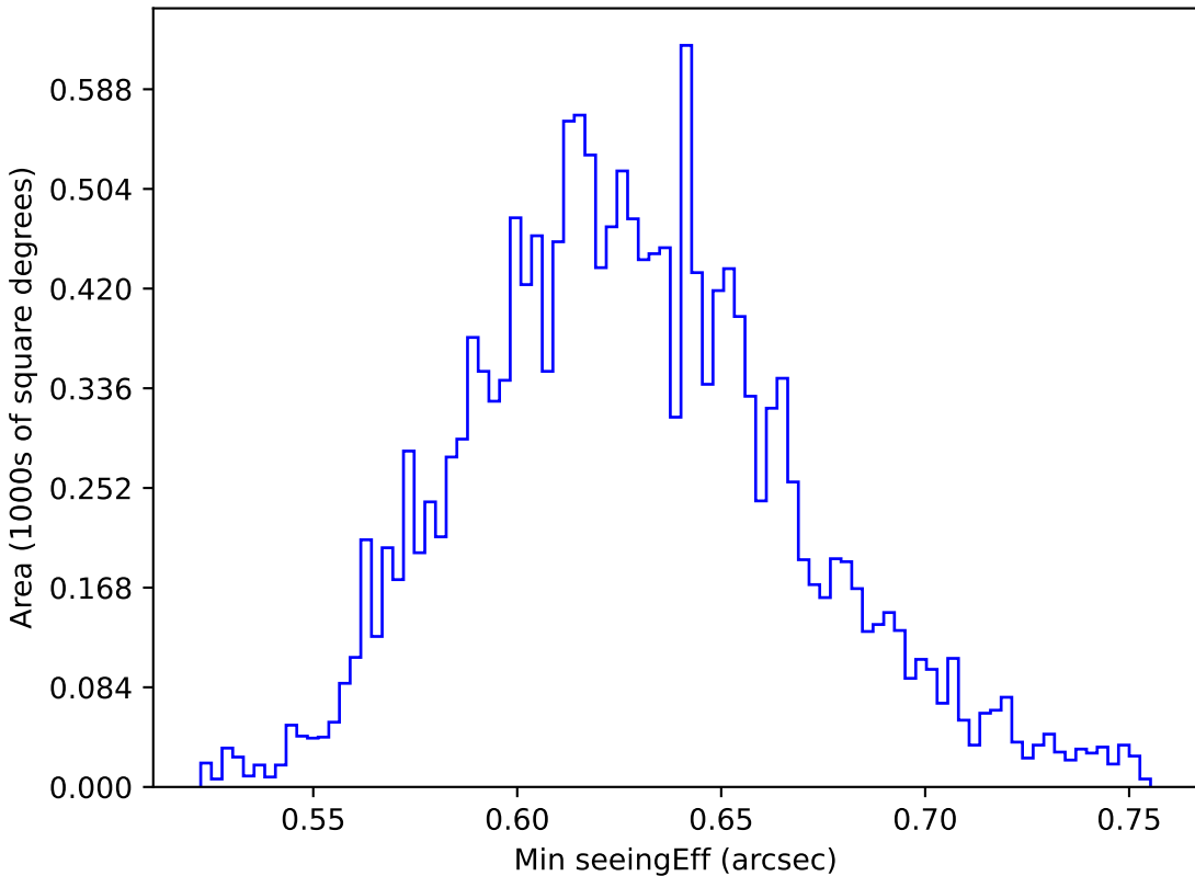
noroll_mjdp180_v3.4_10yrs WFD y band: Min seeingEff
