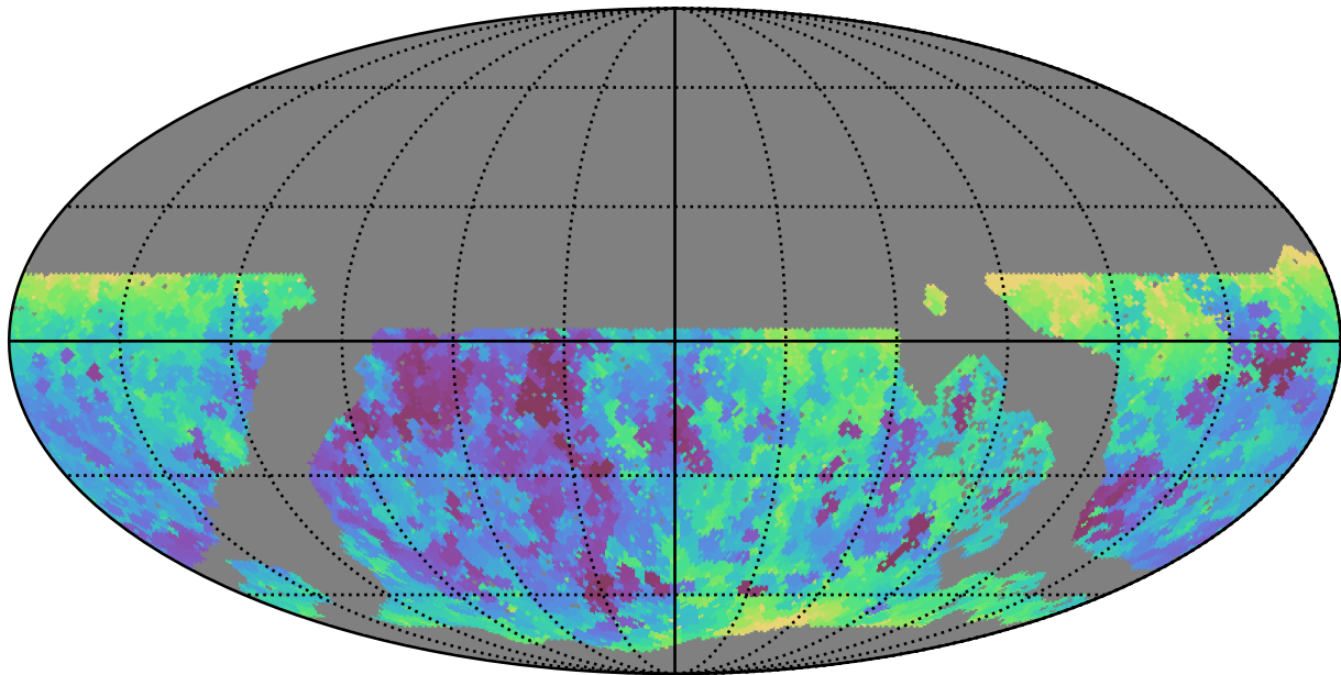
noroll_mjdp180_v3.4_10yrs WFD r band: Min seeingEff
