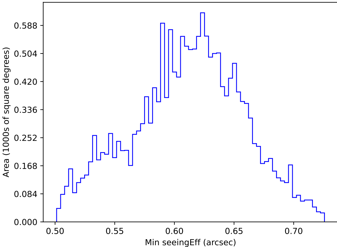
noroll_mjdp180_v3.4_10yrs WFD r band: Min seeingEff
