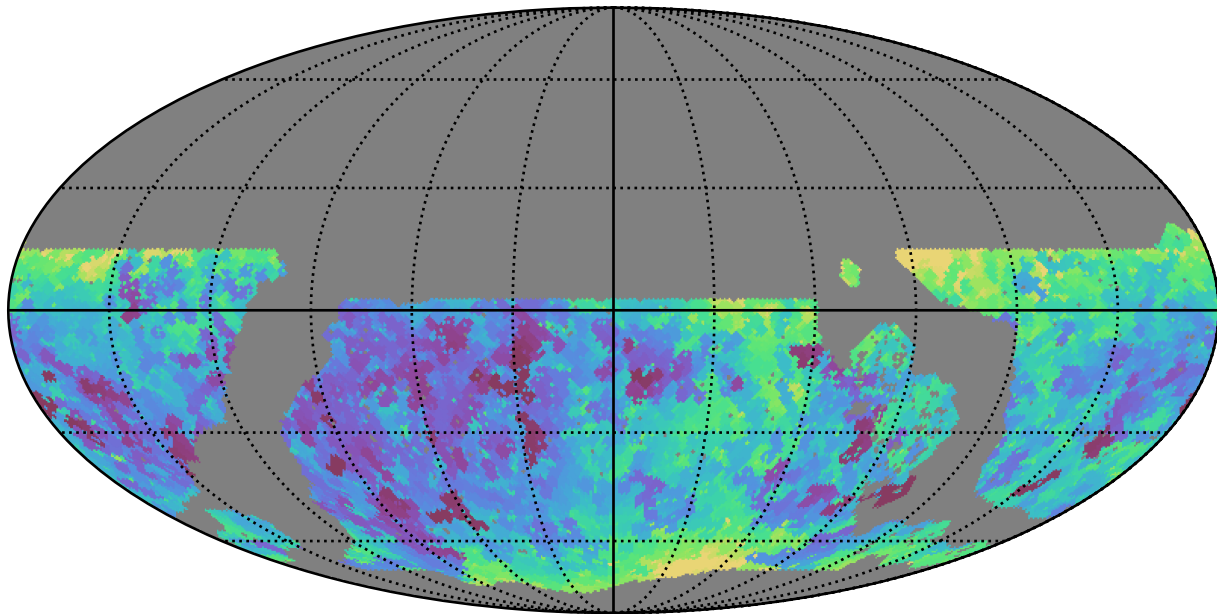
noroll_mjdp180_v3.4_10yrs WFD i band: Min seeingEff
