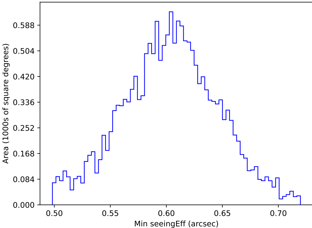
noroll_mjdp180_v3.4_10yrs WFD i band: Min seeingEff
