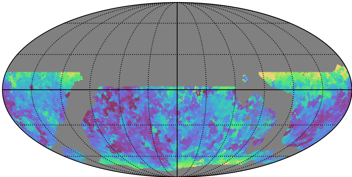
noroll_mjdp180_v3.4_10yrs WFD g band: Min seeingEff
