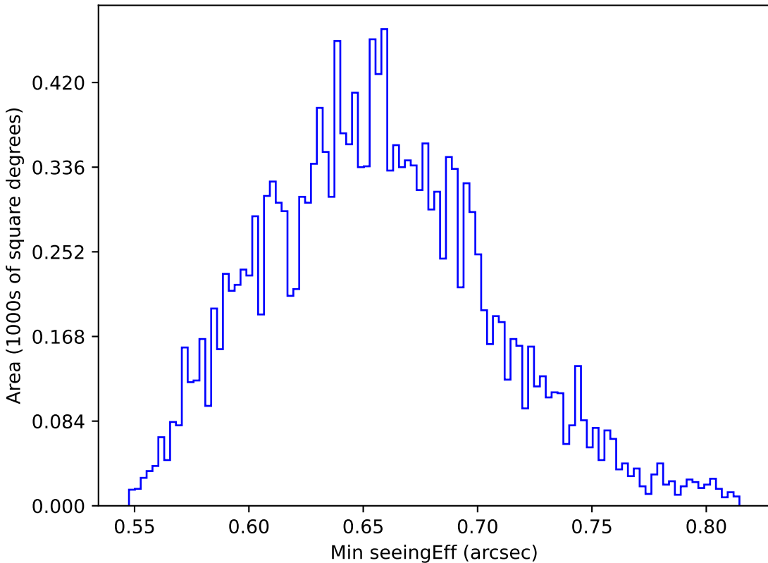
noroll_mjdp180_v3.4_10yrs WFD g band: Min seeingEff
