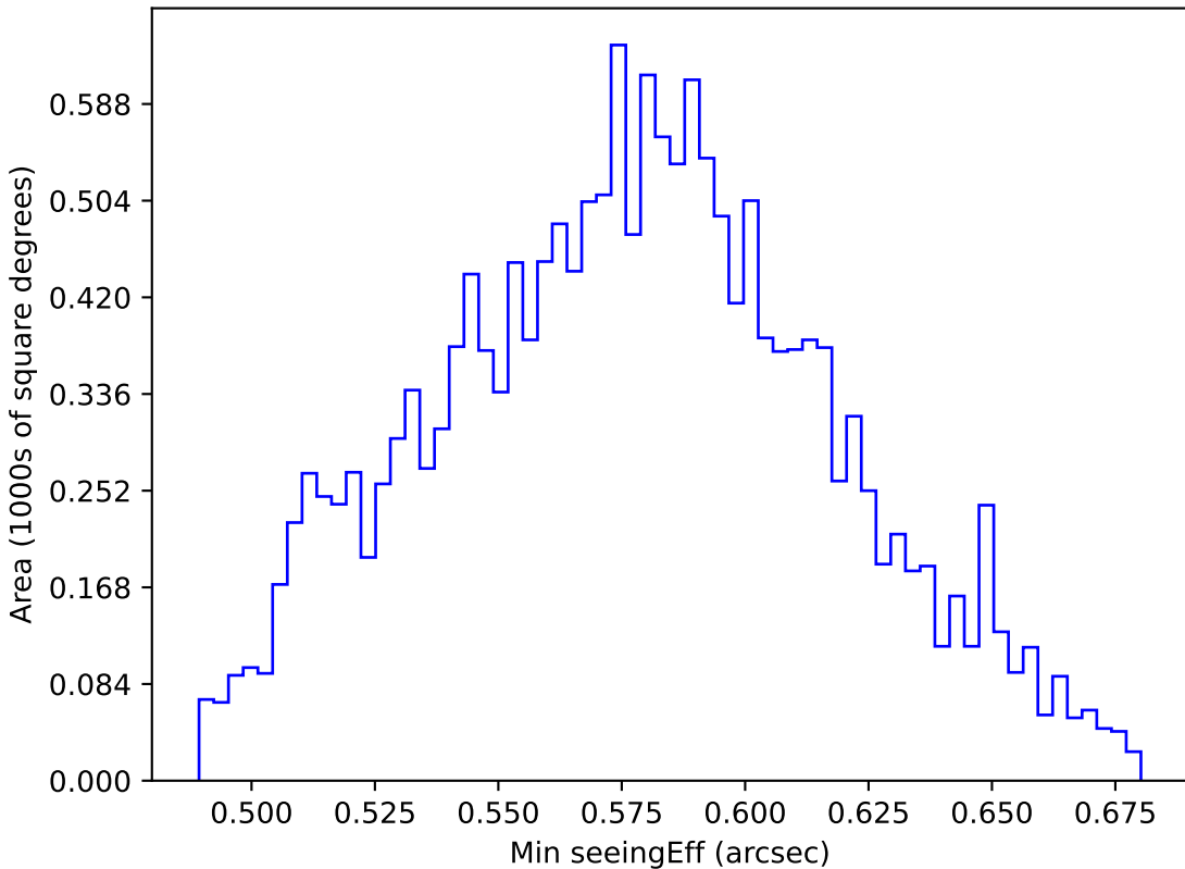
noroll_mjdp180_v3.4_10yrs WFD all bands: Min seeingEff
