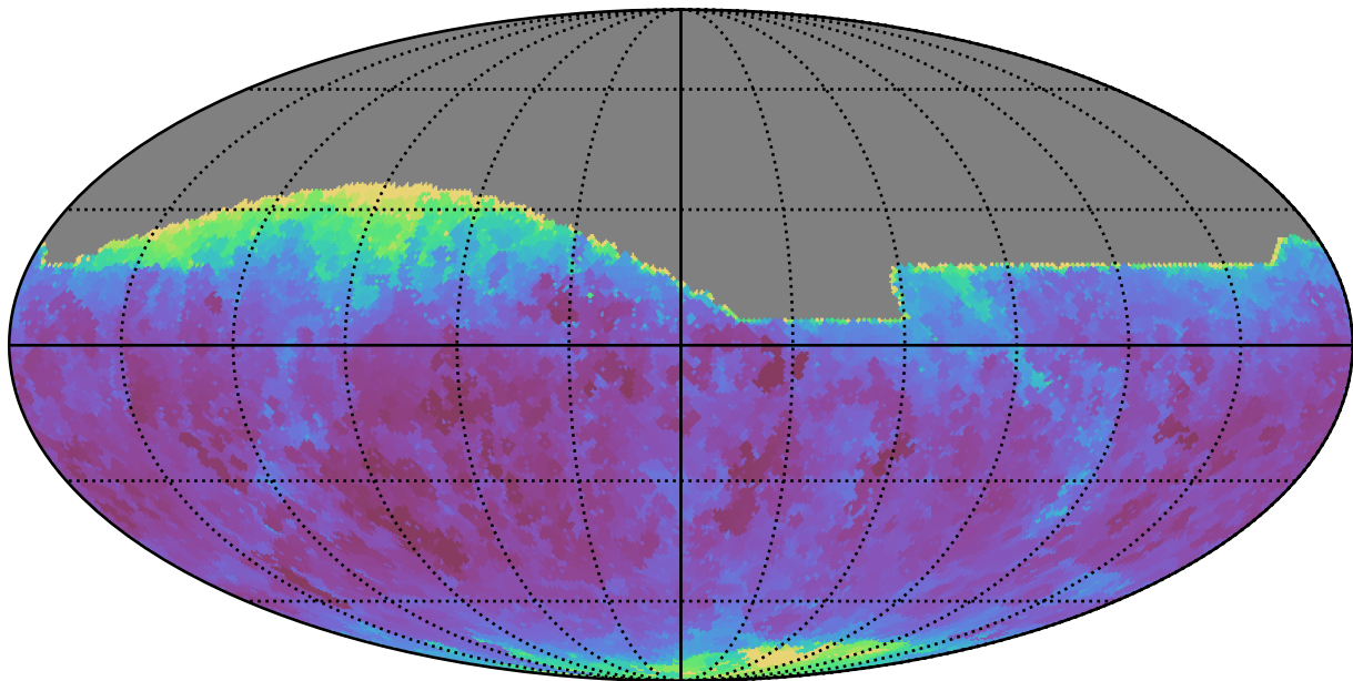
noroll_mjdp180_v3.4_10yrs All sky z band: Min seeingEff
