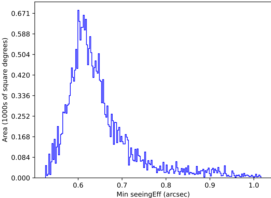
noroll_mjdp180_v3.4_10yrs All sky z band: Min seeingEff
