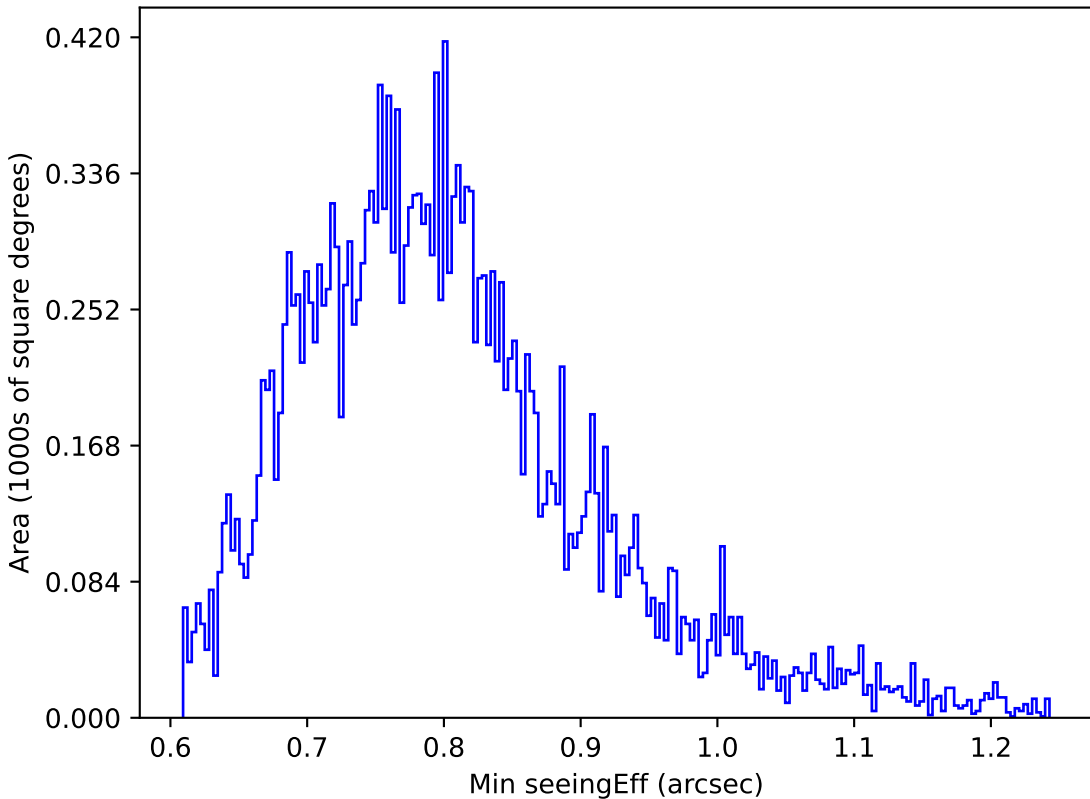
noroll_mjdp180_v3.4_10yrs All sky u band: Min seeingEff
