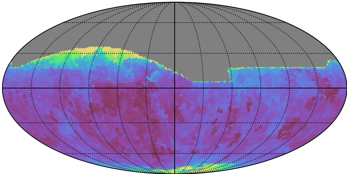
noroll_mjdp180_v3.4_10yrs All sky r band: Min seeingEff
