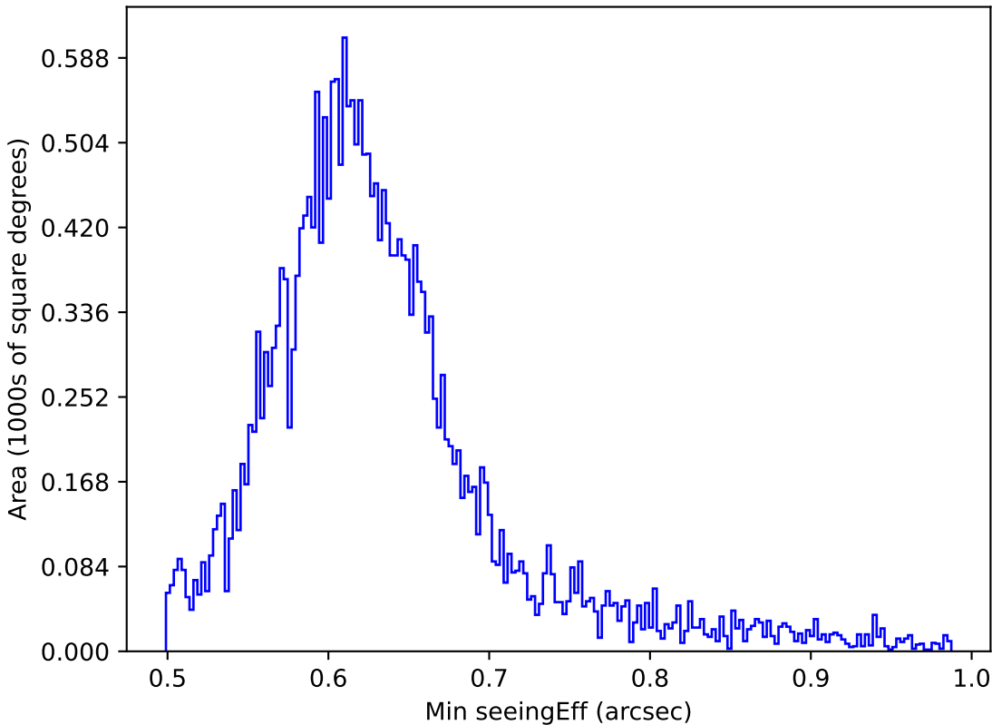
noroll_mjdp180_v3.4_10yrs All sky i band: Min seeingEff
