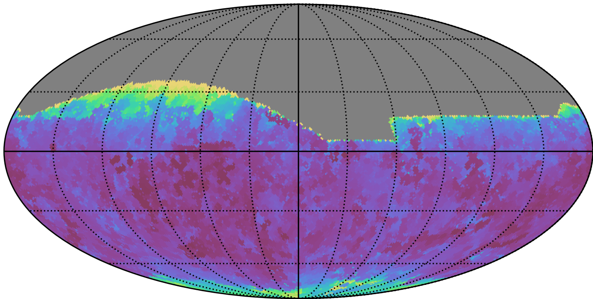
noroll_mjdp180_v3.4_10yrs All sky g band: Min seeingEff
