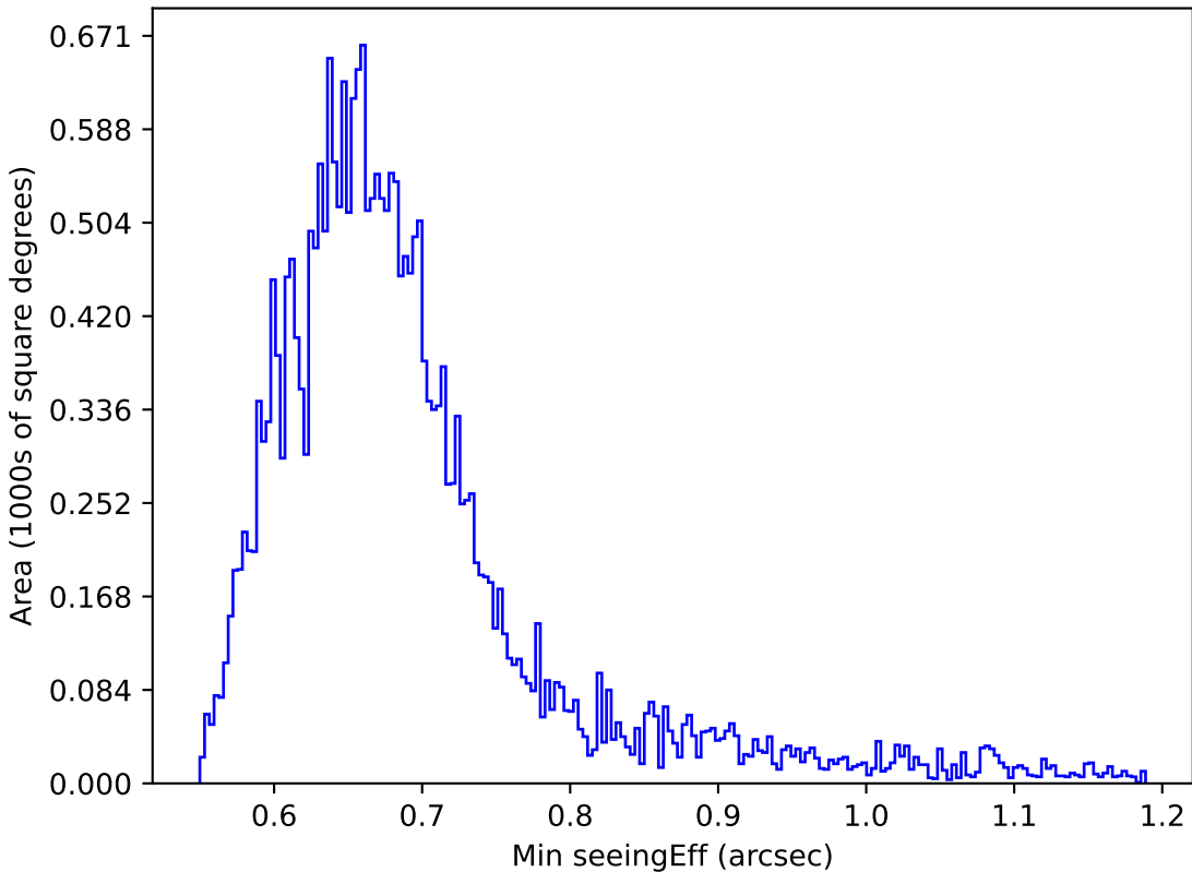
noroll_mjdp180_v3.4_10yrs All sky g band: Min seeingEff
