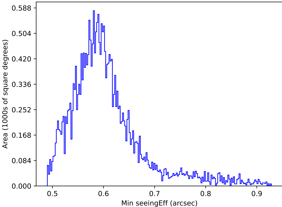
noroll_mjdp180_v3.4_10yrs All sky all bands: Min seeingEff
