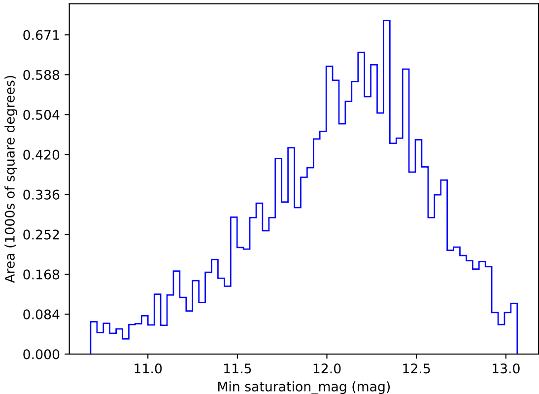
noroll_mjdp180_v3.4_10yrs WFD z band: Min saturation_mag
