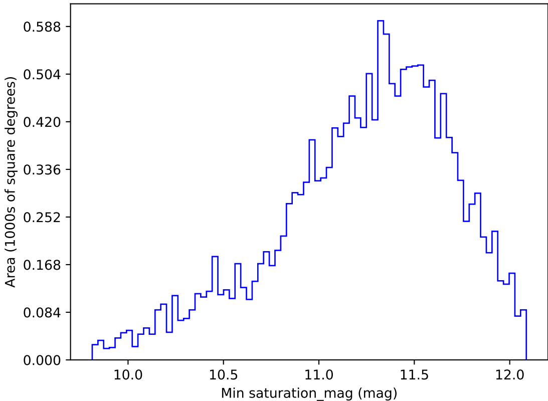
noroll_mjdp180_v3.4_10yrs WFD y band: Min saturation_mag
