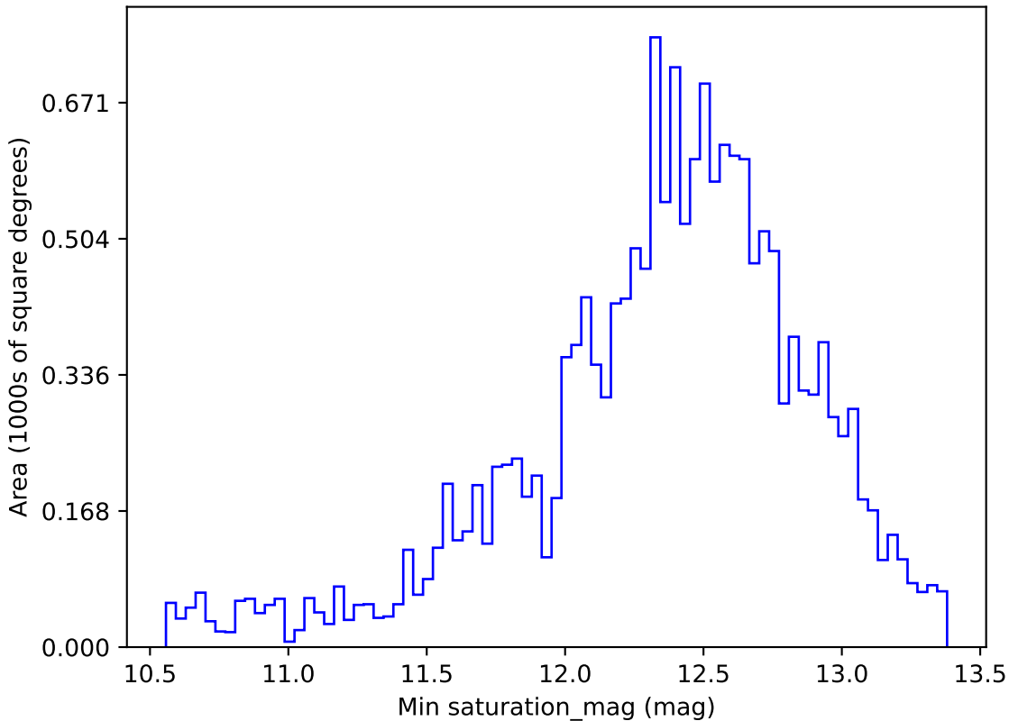
noroll_mjdp180_v3.4_10yrs WFD i band: Min saturation_mag
