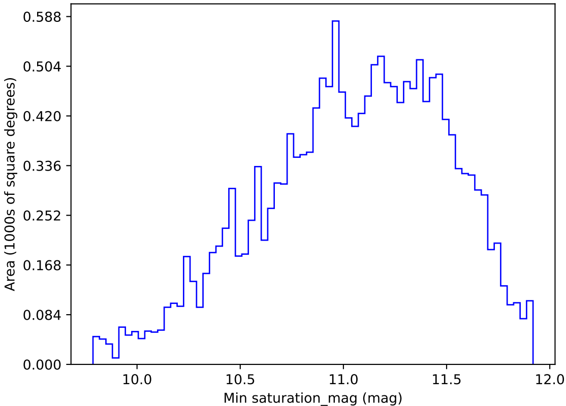
noroll_mjdp180_v3.4_10yrs WFD all bands: Min saturation_mag
