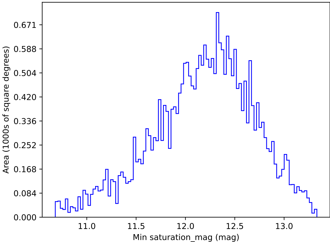
noroll_mjdp180_v3.4_10yrs All sky z band: Min saturation_mag
