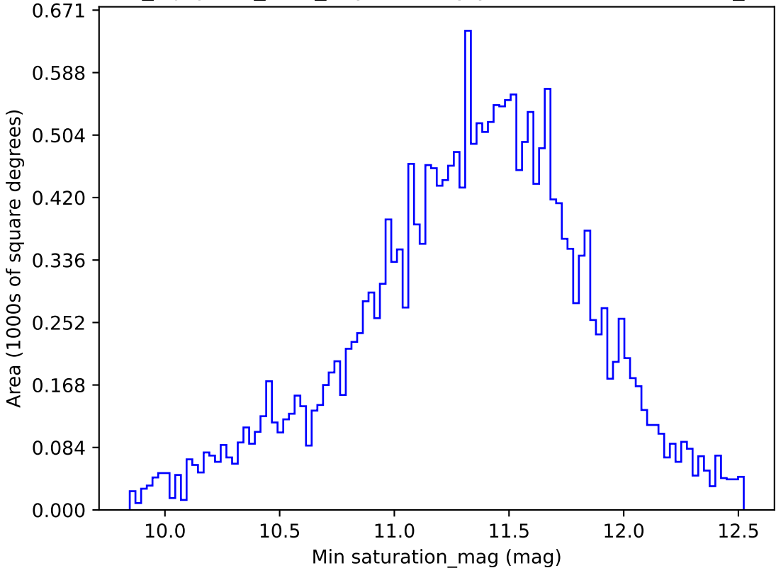
noroll_mjdp180_v3.4_10yrs All sky y band: Min saturation_mag
