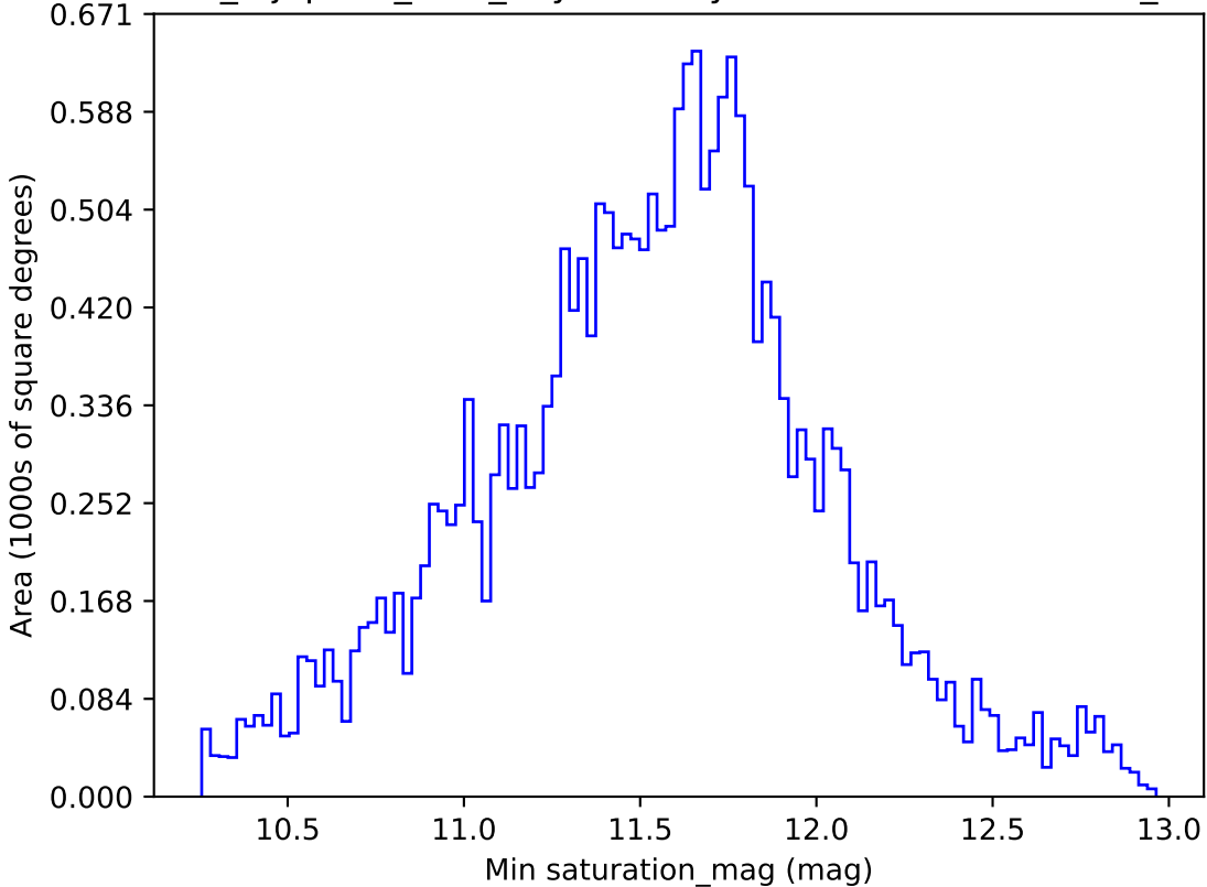
noroll_mjdp180_v3.4_10yrs All sky u band: Min saturation_mag
