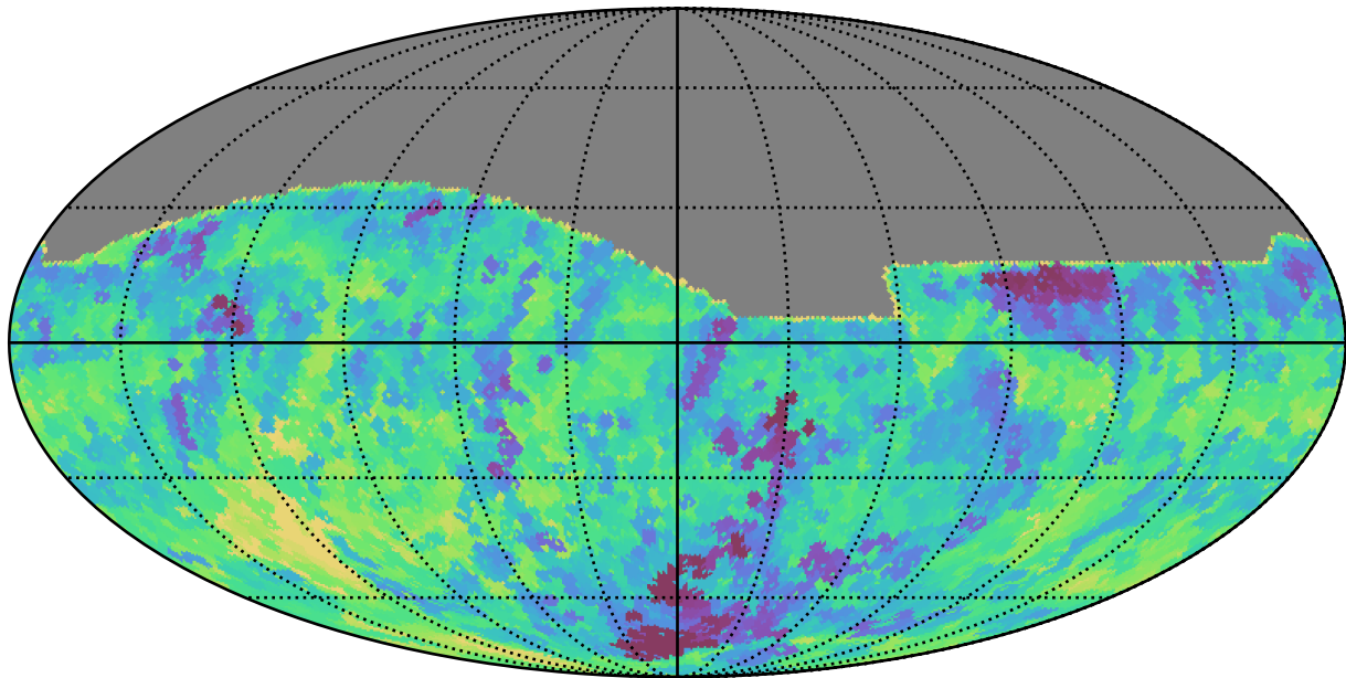
noroll_mjdp180_v3.4_10yrs All sky r band: Min saturation_mag
