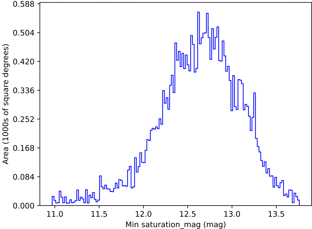
noroll_mjdp180_v3.4_10yrs All sky r band: Min saturation_mag
