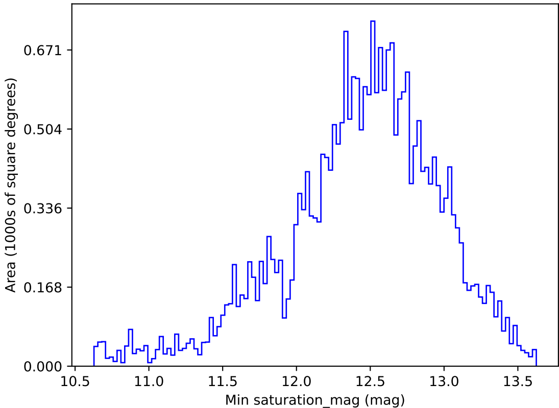
noroll_mjdp180_v3.4_10yrs All sky i band: Min saturation_mag
