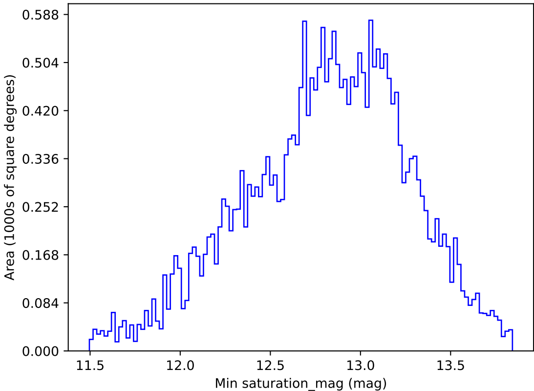
noroll_mjdp180_v3.4_10yrs All sky g band: Min saturation_mag
