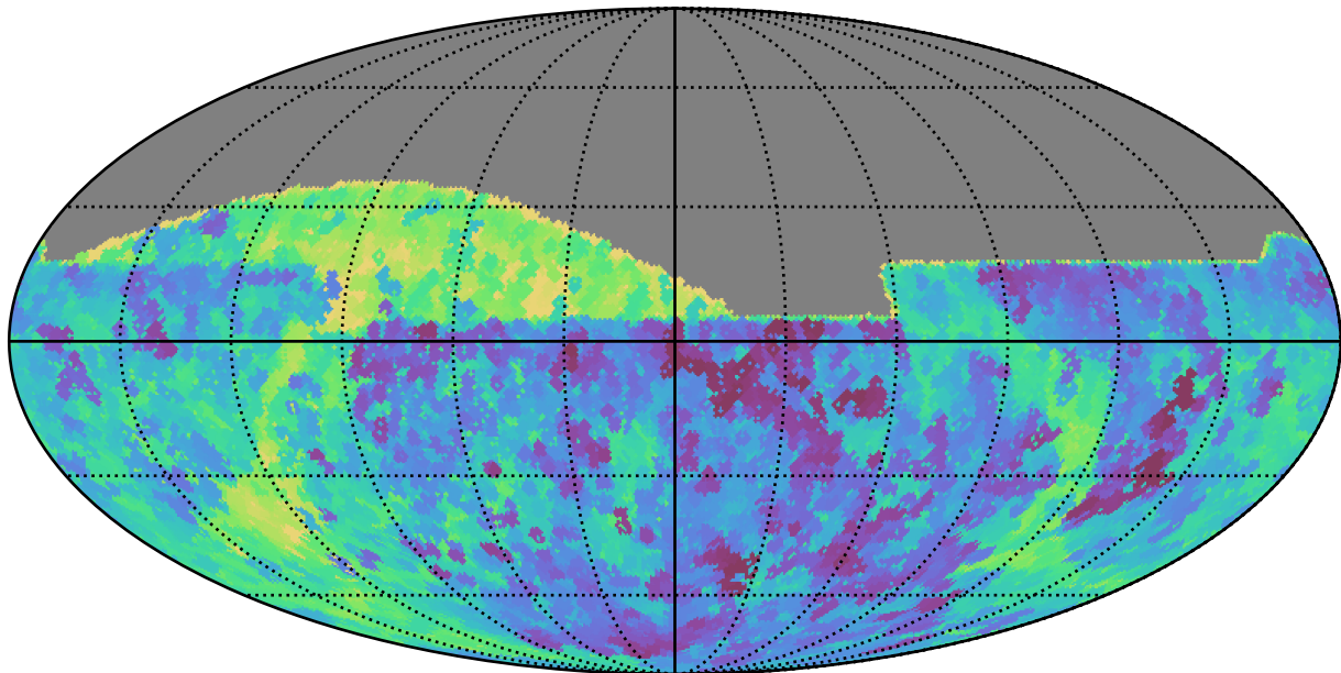
noroll_mjdp180_v3.4_10yrs All sky all bands: Min saturation_mag
