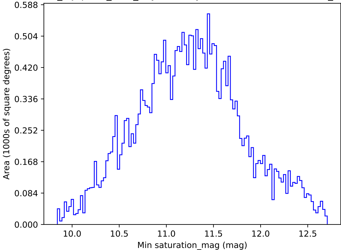
noroll_mjdp180_v3.4_10yrs All sky all bands: Min saturation_mag
