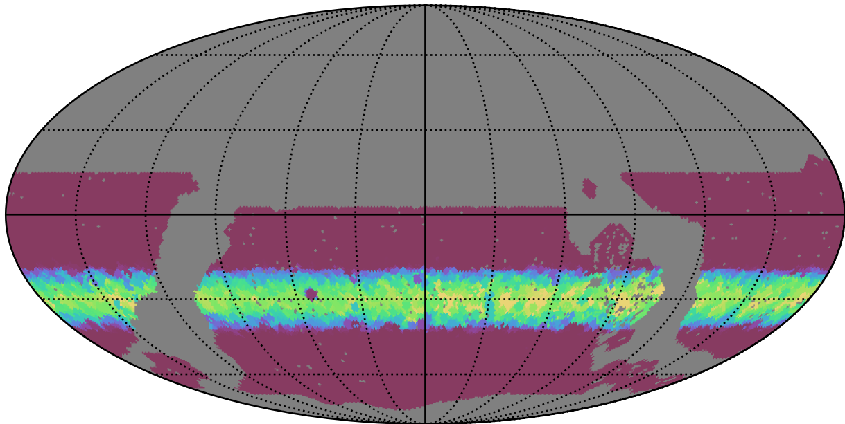
noroll_mjdp180_v3.4_10yrs WFD z band: Min normairmass
