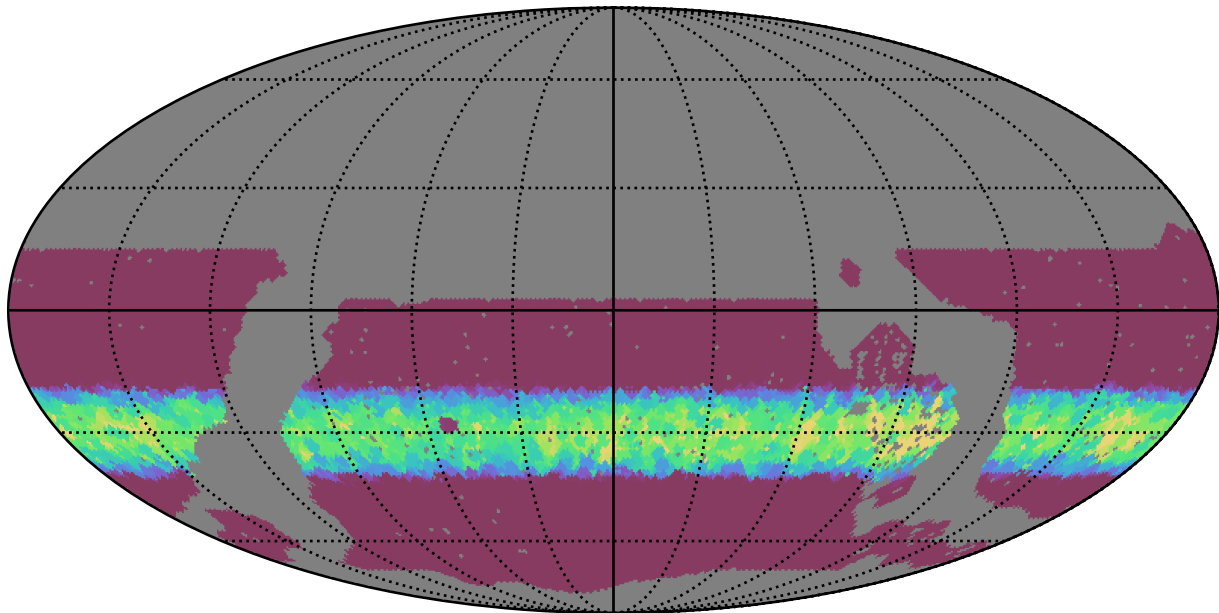
noroll_mjdp180_v3.4_10yrs WFD y band: Min normairmass
