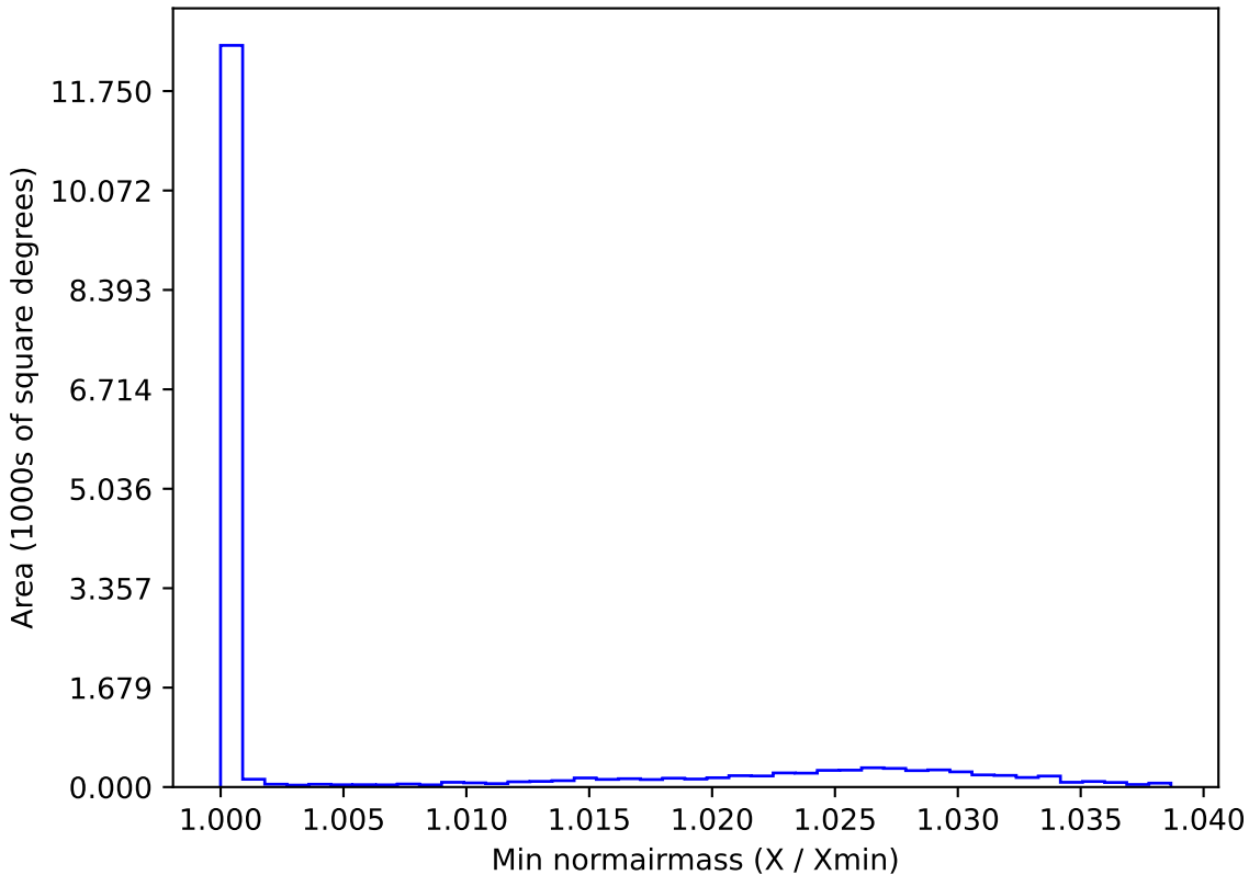
noroll_mjdp180_v3.4_10yrs WFD y band: Min normairmass
