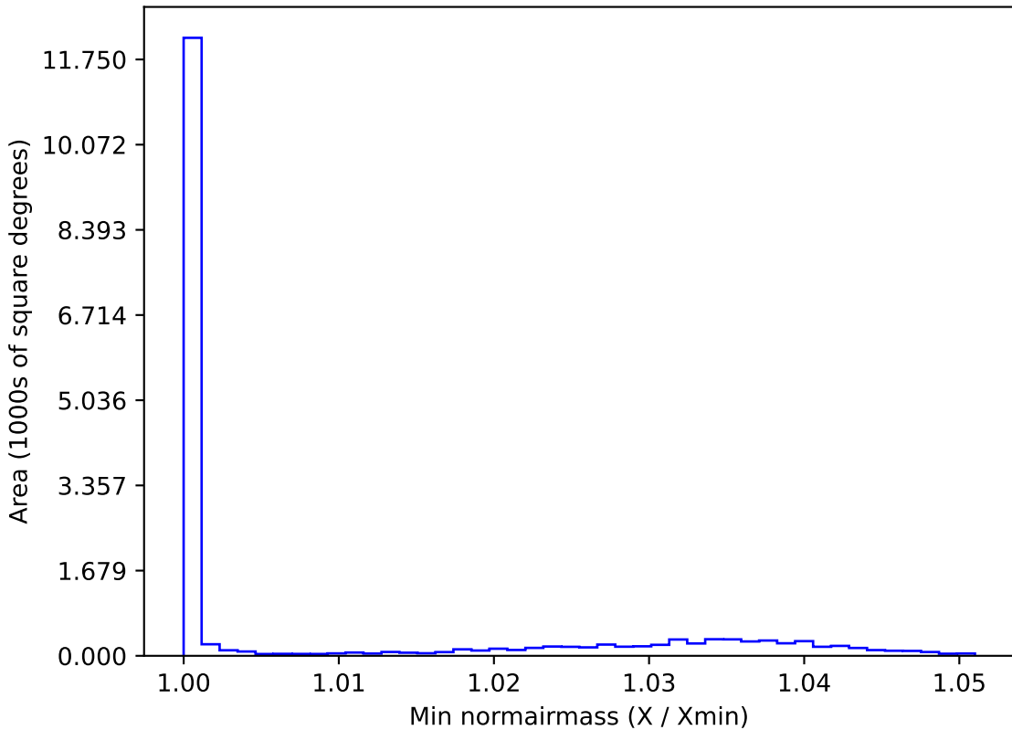
noroll_mjdp180_v3.4_10yrs WFD u band: Min normairmass
