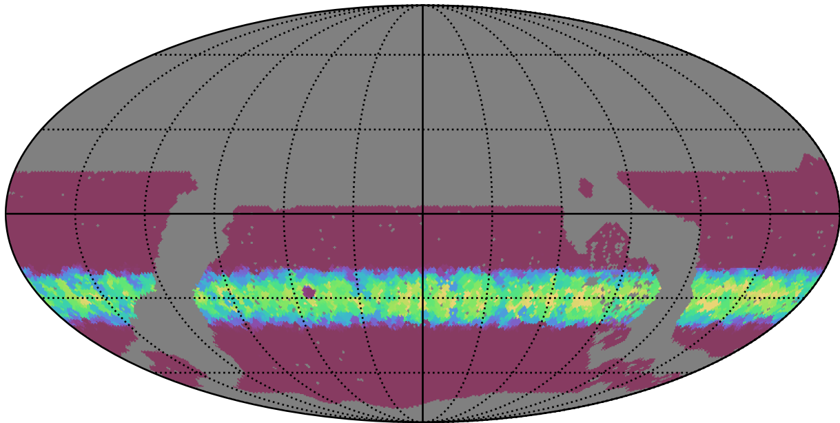
noroll_mjdp180_v3.4_10yrs WFD r band: Min normairmass
