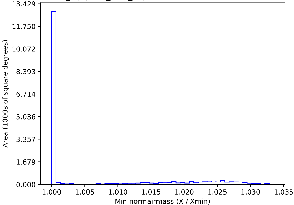
noroll_mjdp180_v3.4_10yrs WFD r band: Min normairmass
