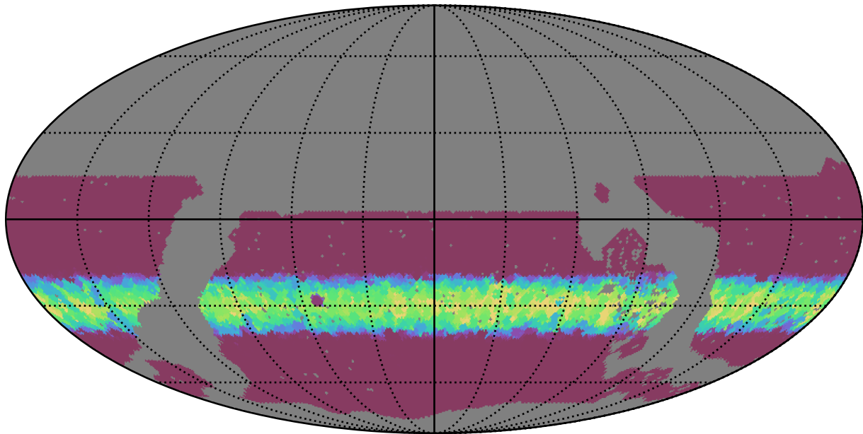
noroll_mjdp180_v3.4_10yrs WFD i band: Min normairmass
