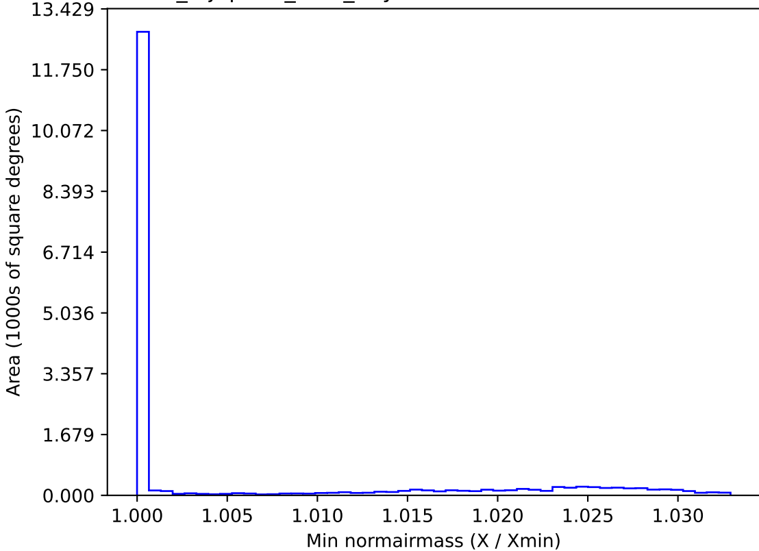
noroll_mjdp180_v3.4_10yrs WFD i band: Min normairmass
