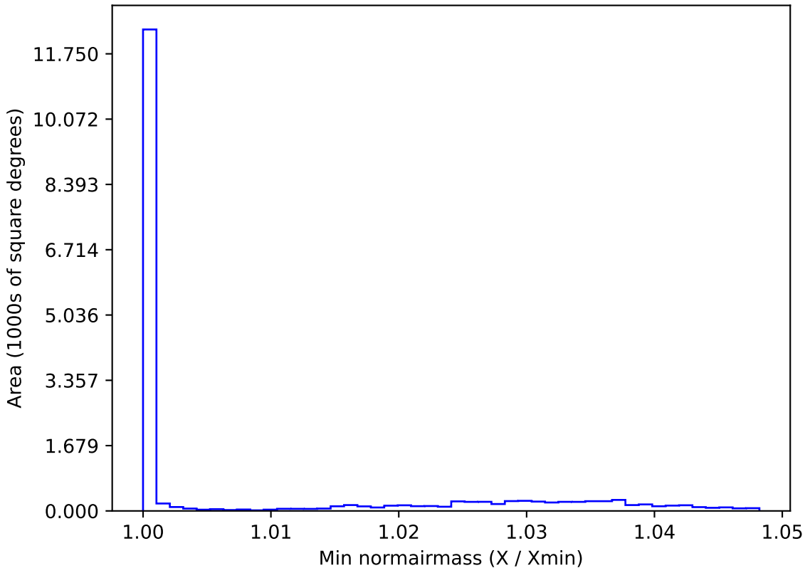
noroll_mjdp180_v3.4_10yrs WFD g band: Min normairmass
