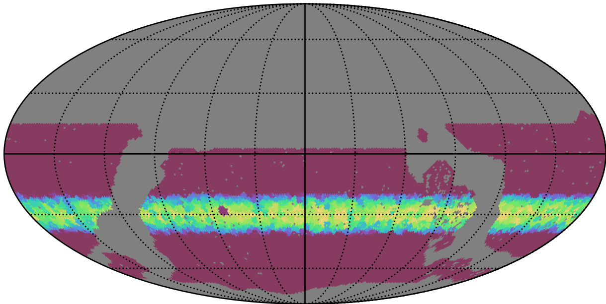
noroll_mjdp180_v3.4_10yrs WFD all bands: Min normairmass
