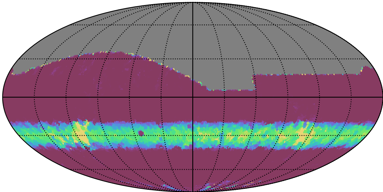
noroll_mjdp180_v3.4_10yrs All sky z band: Min normairmass
