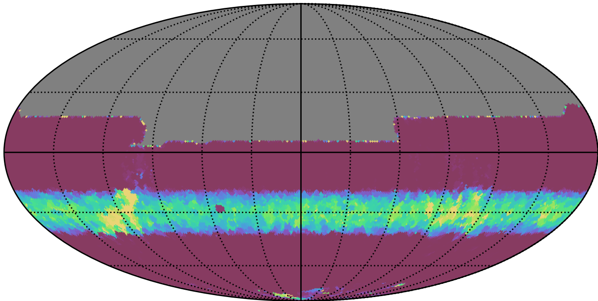
noroll_mjdp180_v3.4_10yrs All sky y band: Min normairmass
