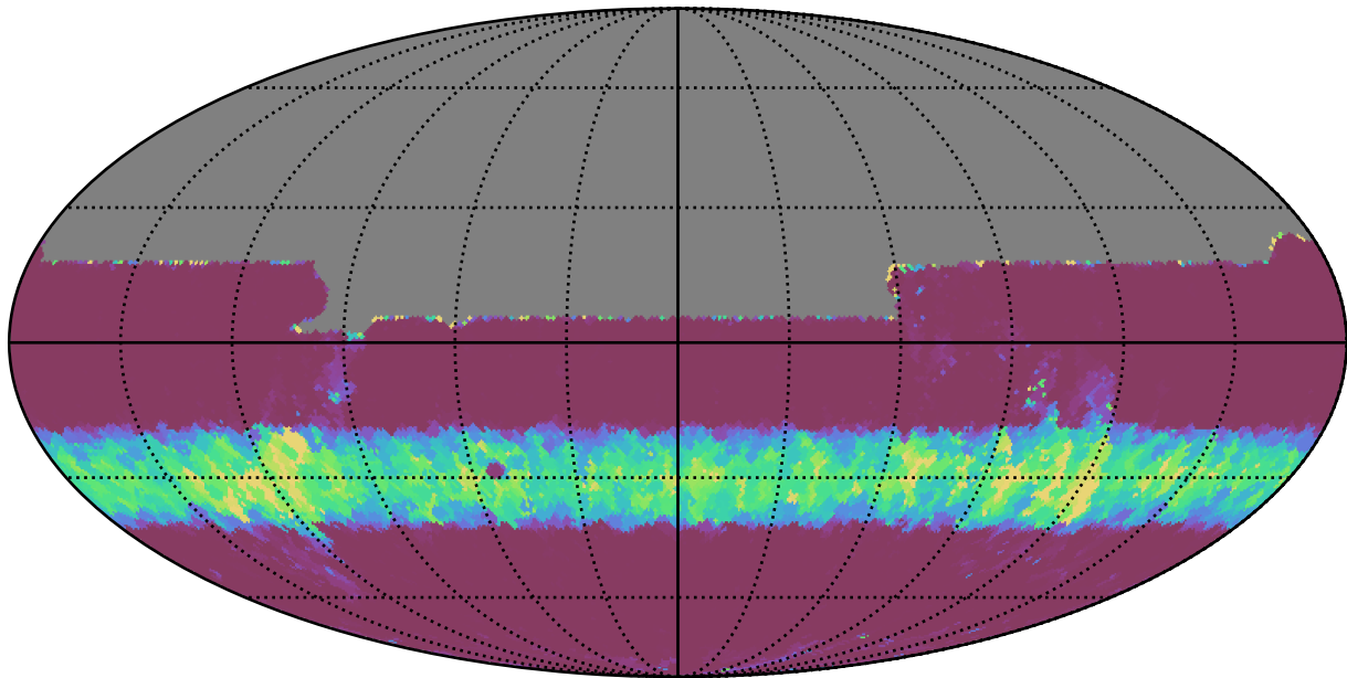
noroll_mjdp180_v3.4_10yrs All sky u band: Min normairmass
