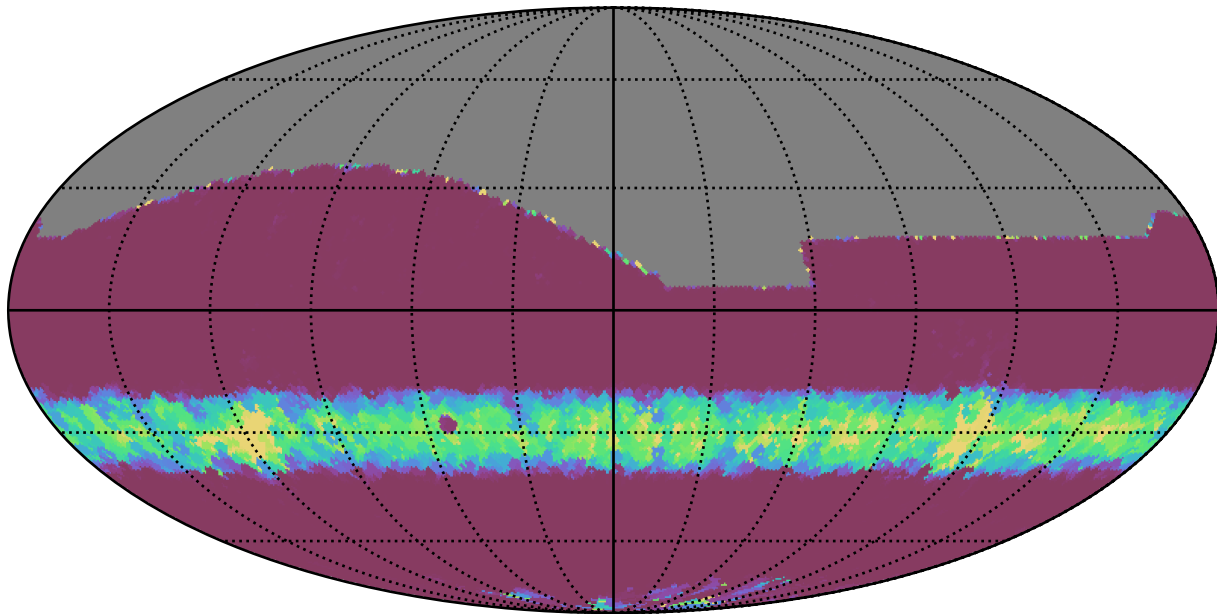
noroll_mjdp180_v3.4_10yrs All sky r band: Min normairmass
