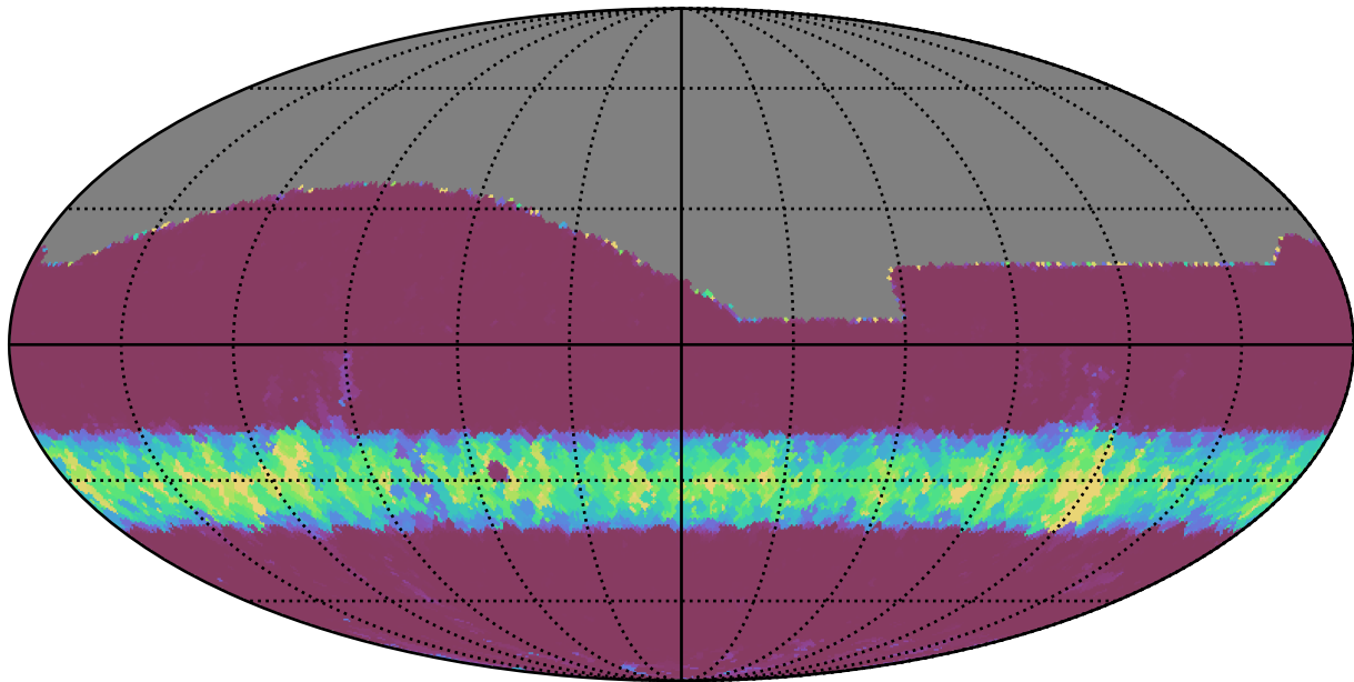
noroll_mjdp180_v3.4_10yrs All sky g band: Min normairmass
