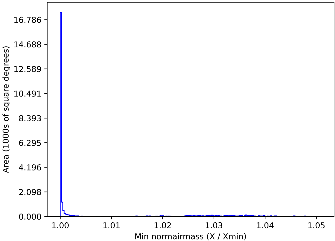
noroll_mjdp180_v3.4_10yrs All sky g band: Min normairmass
